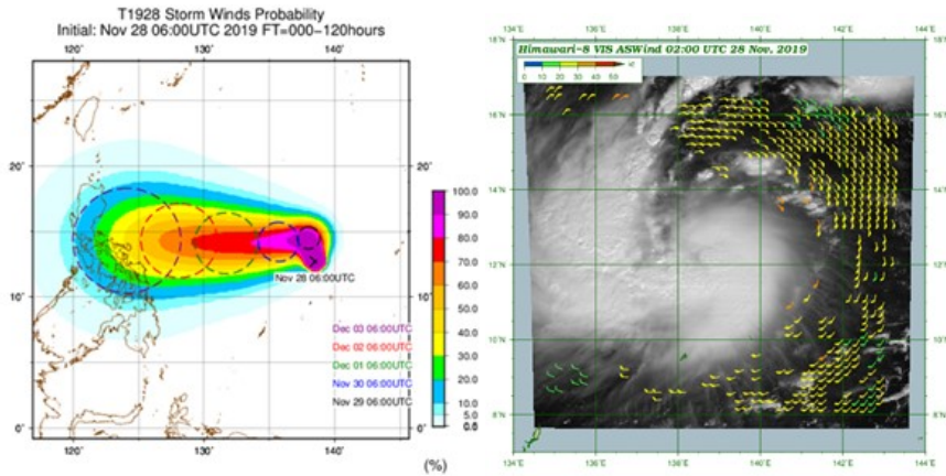
(Left) Storm Wind Probability Map: Probabilistic forecast map for sustained wind equal to or above 50-kt with forecast time of 1, 2, 3, 4 and 5 days, to grasp the possible impact for areas of interest. (Right) Sea-surface AMV: AMV-based sea-surface wind in the vicinity of TCs estimated from Himawari-8/9 low-level AMVs. Data are available every 30 minutes for full-disk observation and every 10 minutes for Target Area observation, respectively.
